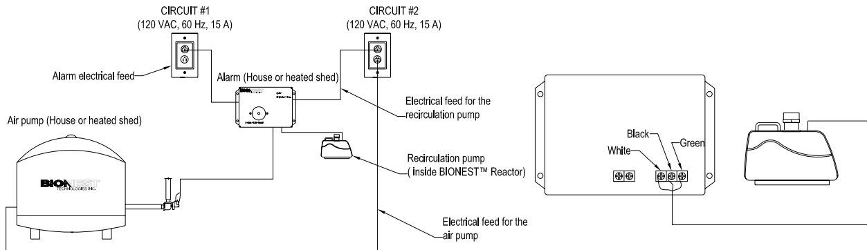
FIGURE 4: ELECTRICAL CONNECTION
