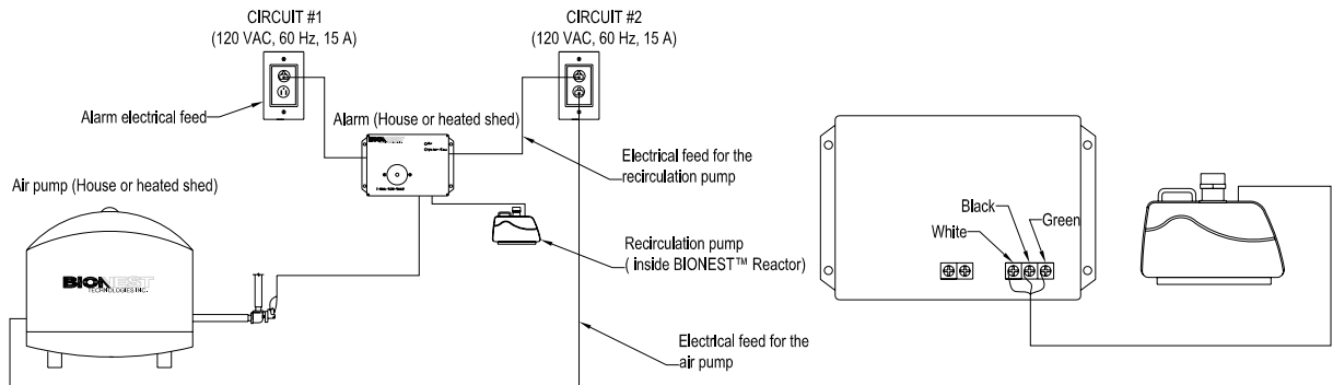
FIGURE 4: ELECTRICAL CONNECTION
